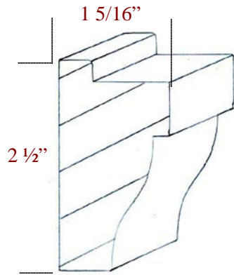
C-595 7/8x1/4" notch
