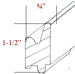
C-506 Drawer Pull
