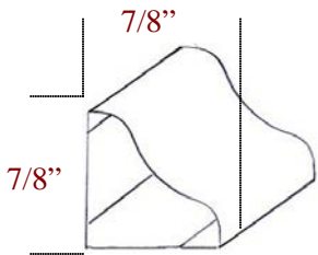
S-552 Shoe Molding
