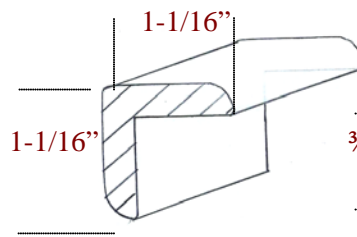
S-513 (S-513B 1x1) Outside Corner
