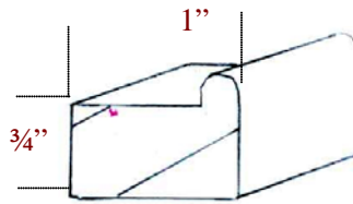
C-596 shelf edge 3/4 x 1/4" notch
