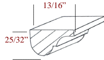
S-519 Hutch Top
