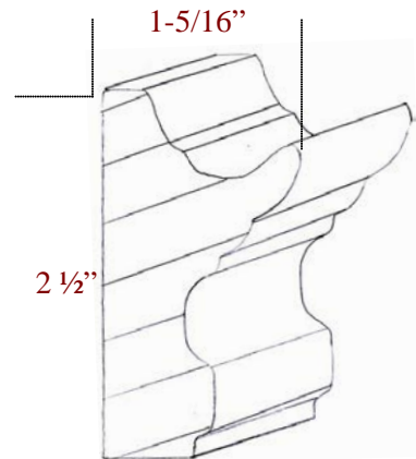
C-522 Picture Rail/Plate Rail (wall mount)
