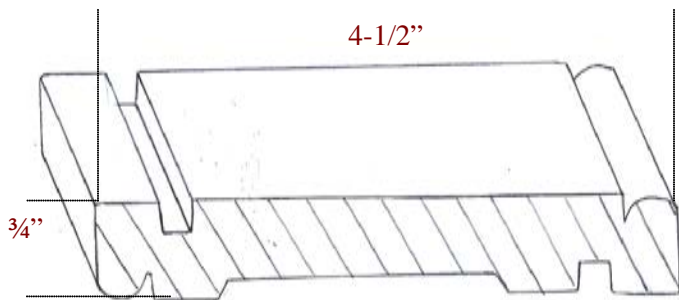
S-512 Reversible Freize Board
